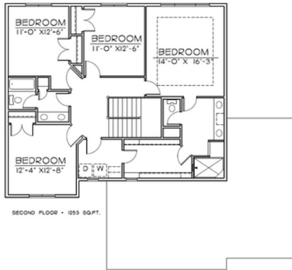
Second Floor Layout
